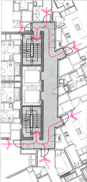
APARTMENT LEVELS ESCAPE PATHS
