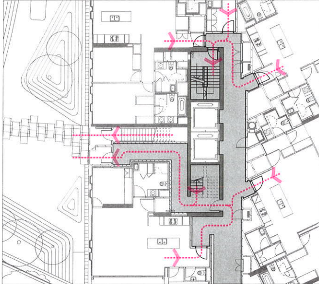
LEVEL 1 ESCAPE PATHS
