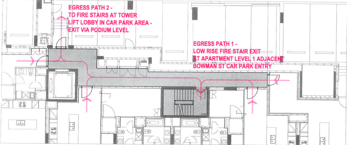
LOW RISE APARTMENT LEVELS ESCAPE PATHS
